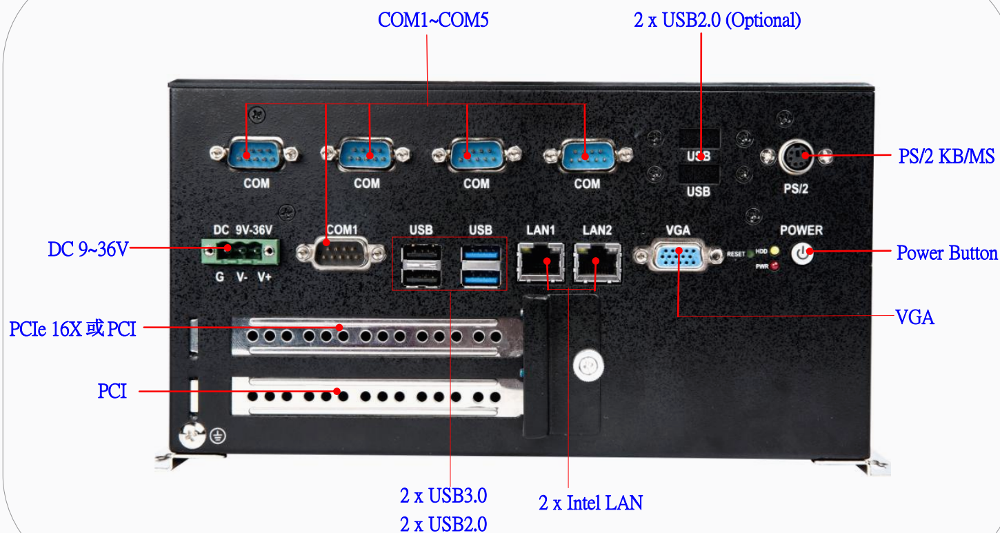
Front I/O View
